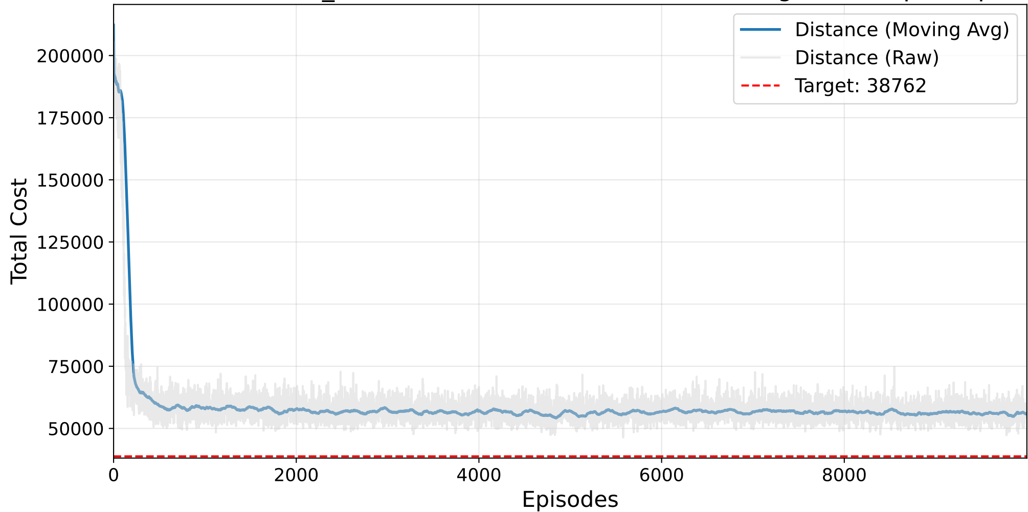
Final RANDOM_SEARCH Masked AutoRL-SOP Training - kro124p.1.sop
